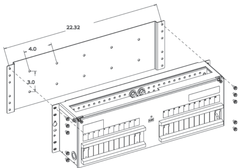
CC848786401 Wall Mounting Bracket for any Panel
