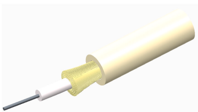
All-Dielectric Indoor/Outdoor Riser Simplex Cable, Reel in Box, 1000 FT
