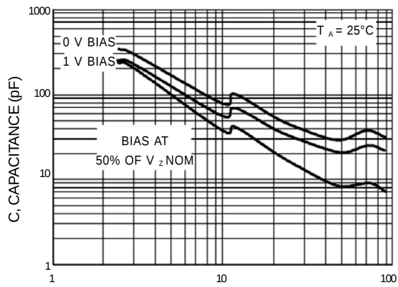
Figure 5. Typical Capacitance
