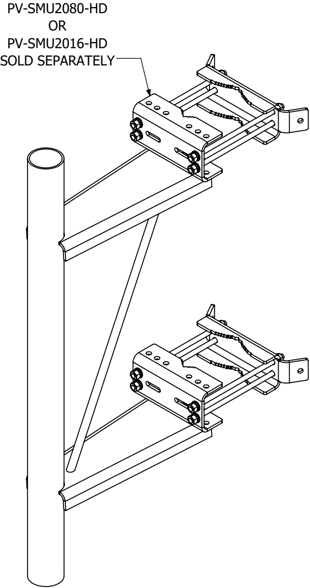
PIPE MOUNT STANDOFF WITH LEG ATTACHMENT BRACKETS
