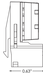
Cat6 Keystones
