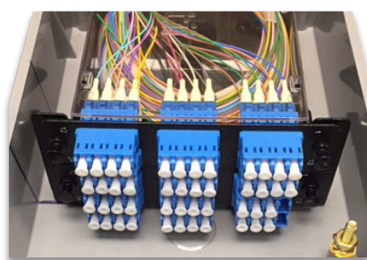
PSC Series Cassette installed inside the 507F Series Enclosure using the BKT-PSC2 Mounting Bracket
