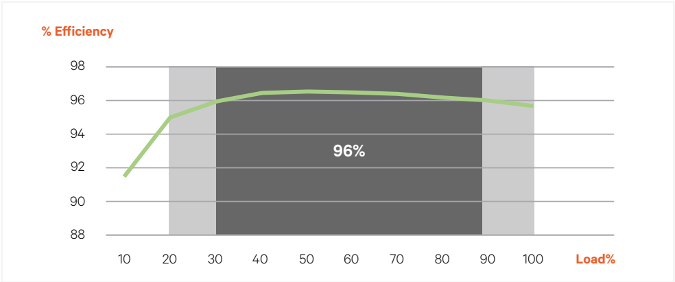
R48-3500e3 Efficiency Curve at 230 VAC Nominal
