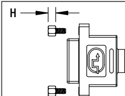
SUPPLIED WITH (4) #4-40 JACKSCREWS FOR PANEL MOUNT 2X H = .160 - PANEL MOUNT HARDWARE 2X H = .191 - CABLE MOUNT HARDWARE
