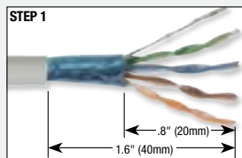
Strip jacketing and shield to dimensions shown.
