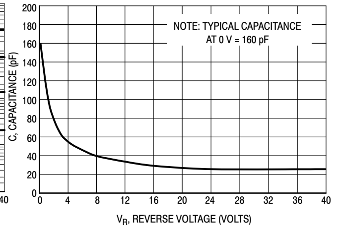
Figure 4. Typical Capacitance
