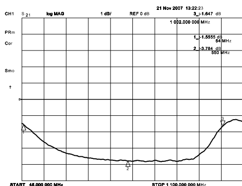
Example Peak-to-Valley Response for Haystacks (727397/789316/761842)
