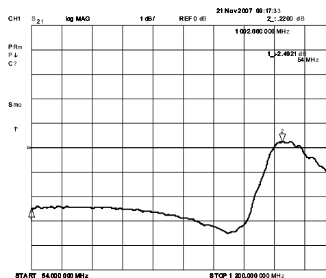
Example Peak-to-Valley Response for Peaking Circuits (727398/761843)
