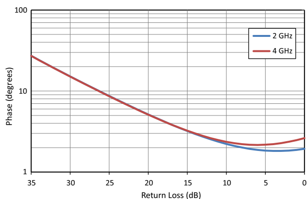
Phase Uncertainty
